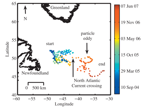
Fig. 1. Trajectory of bio-optical Apex float 0005.
