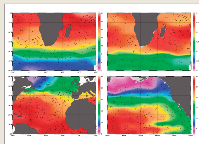
Plots of the distribution of some ocean properties using data acquired during the last ten days of July 2007. Clockwise from top left the plots show sea surface temperature surrounding southern Africa, salinity at a depth of 200 metres, temperature at 100 metres in the North Pacific and sea surface temperature again, this time in the North Atlantic
