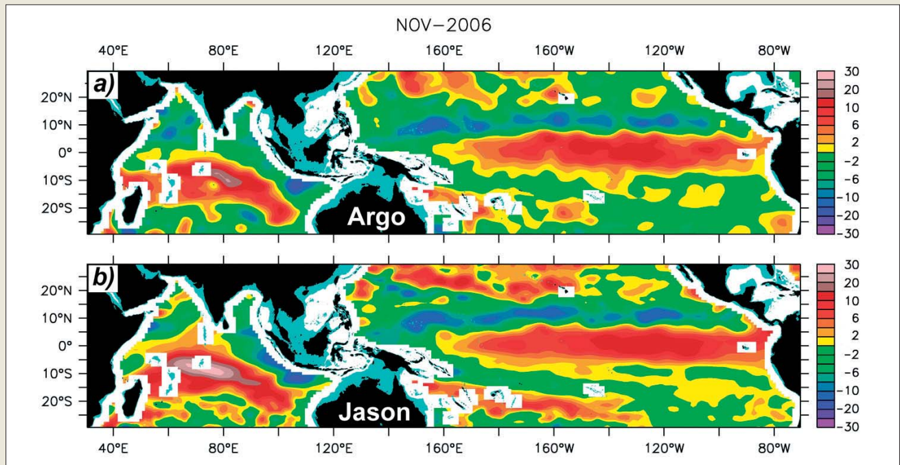
Sea surface height anomaly in November 2006 (cm, relative to a three-year mean 2004-2006) estimated from Argo profile data (a) and from satellite altimetry (b). High values in the eastern equatorial Pacific indicate El Niño conditions
