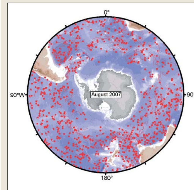
Some of the blank areas close to Antarctica contain floats, but at the time of this image these are under winter ice cover. They will reappear in austral spring
