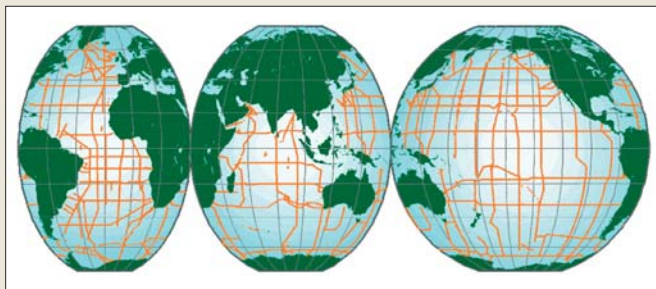
Survey lines occupied during the field programme phase of WOCE
