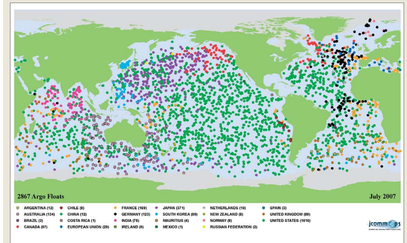
The distribution of floats in the Argo array, July 2007
