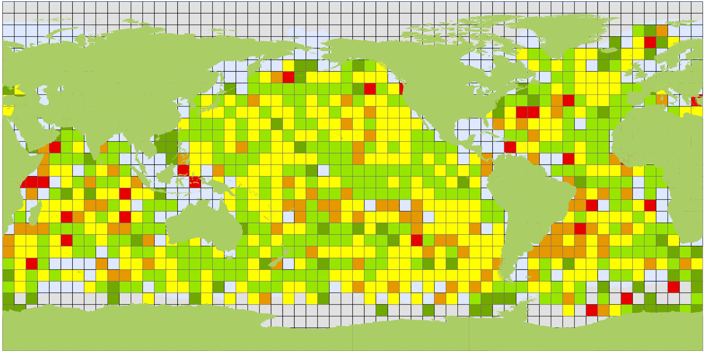
3066 Argo Floats
