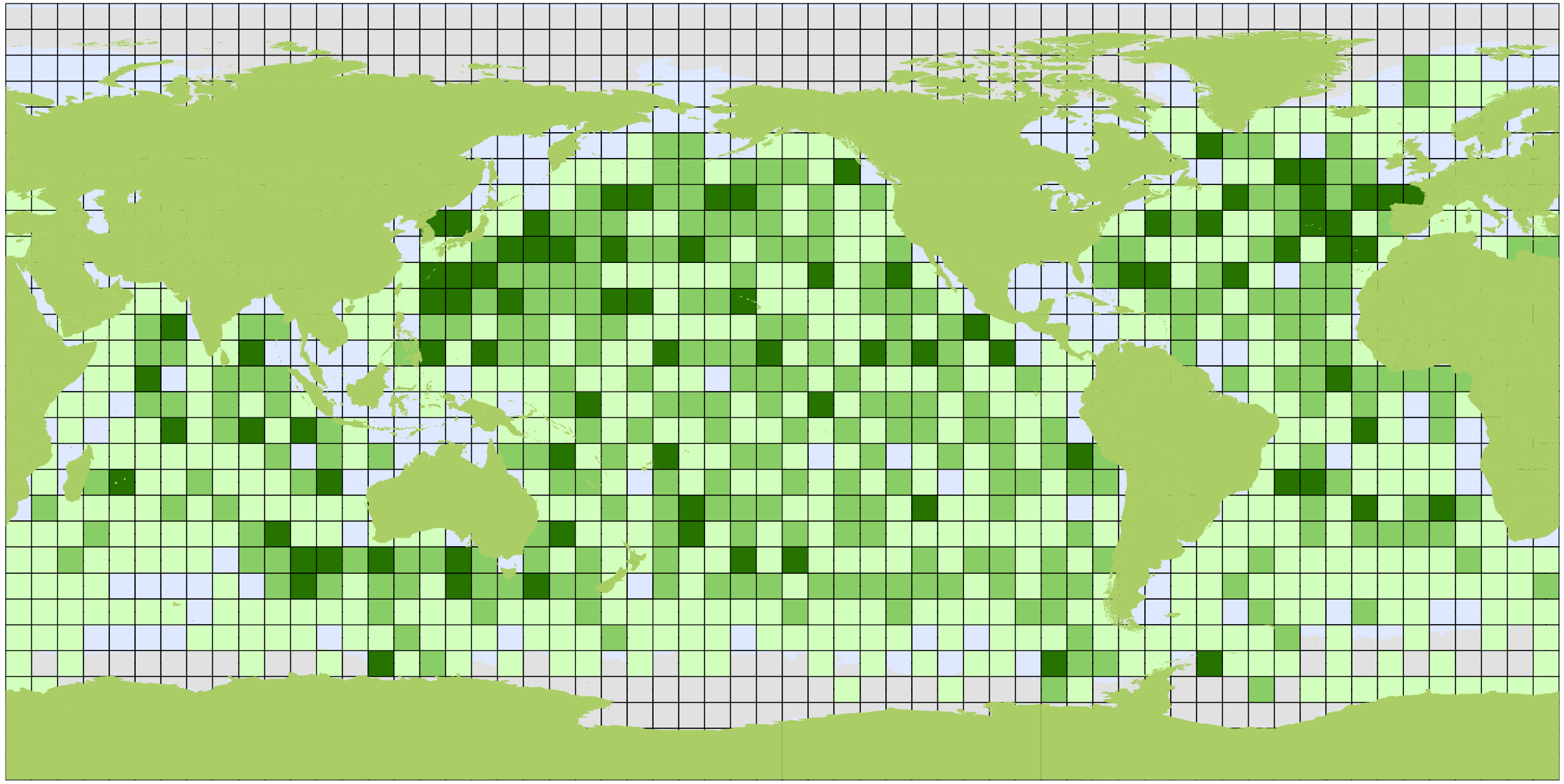
3006 Argo Floats
