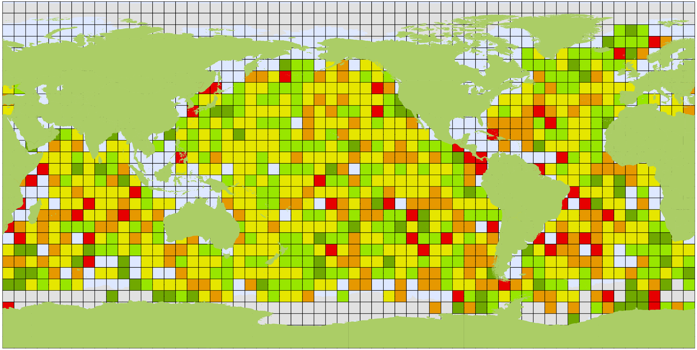
3189 Argo Floats
