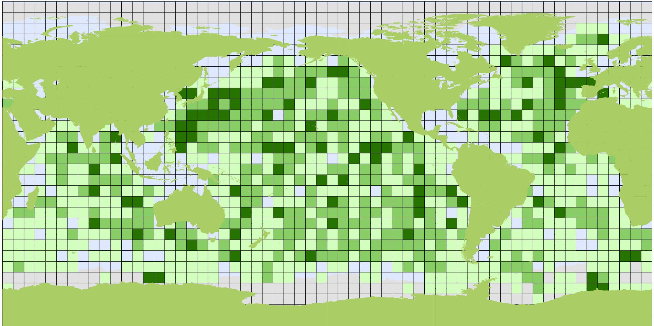
3189 Argo Floats
